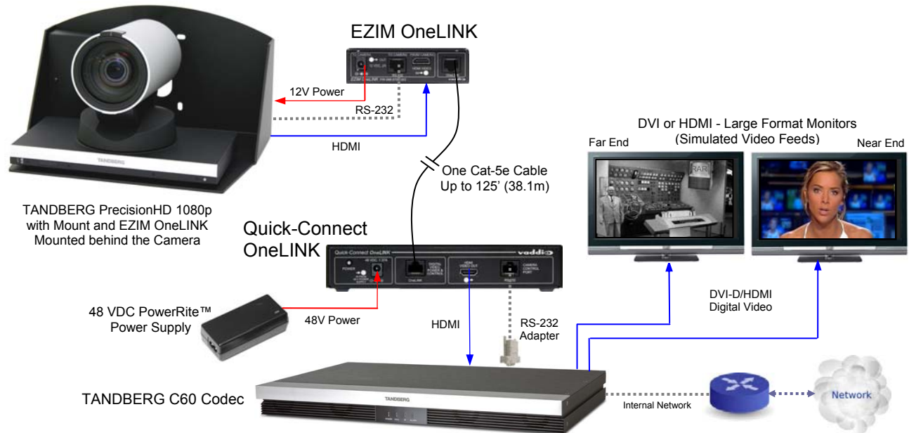
Figure 5: Basic OneLINK System (Quick-Connect and EZIM) Configuration with TANDBERG Camera and Codec
