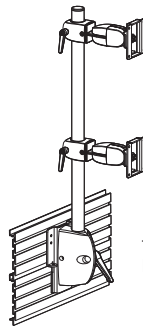
1 1/2" Pole mounted to slatwall with Large Clamp
