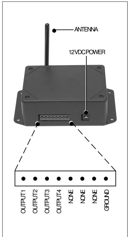
Figure 1 – TouchVIEW Receiver.
