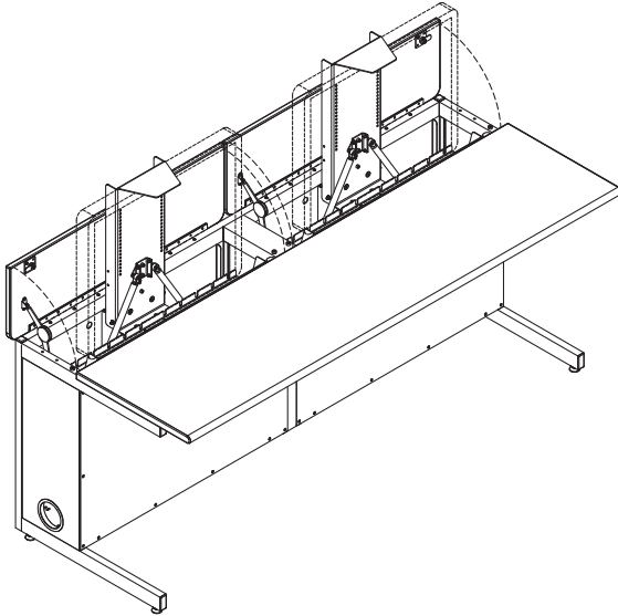
72" Flex Insight XMS double workstation with locking lid
