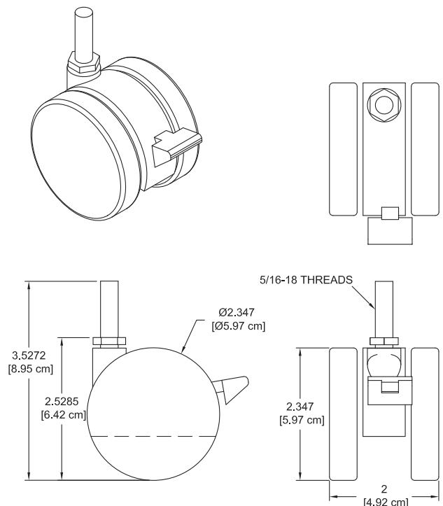
Twin-wheel casters
